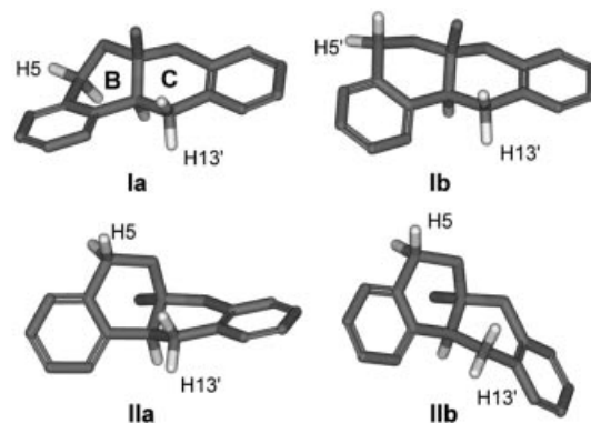
Figure 1. 3D structures of the more stable conformations of the trans and cis diastereoisomers.
