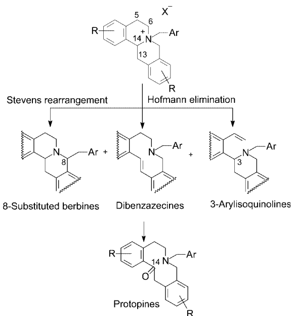
Scheme 2. Reactivity of ( \pm )-berbinium salts under basic conditions.
