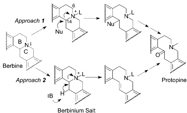
Scheme 1. Approaches to the synthesis of protopine alkaloids.
